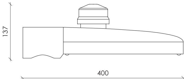
Dimensions with NEMA
