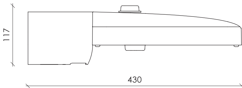
Dimensions with 2 Zhaga connectors
