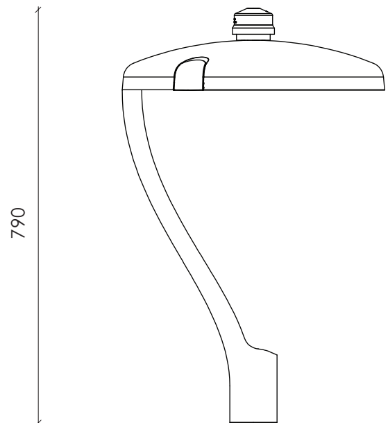
Dimensions with NEMA socket
