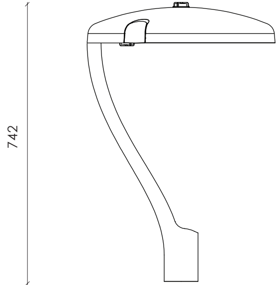
Dimensions with 2 Zhaga connectors
